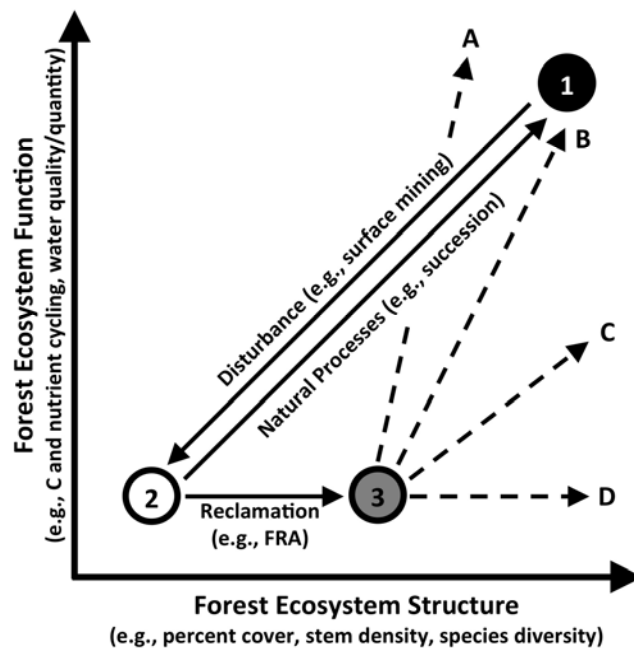
Figure 1. Responses of forest ecosystems in terms of both structure and function as affected by disturbance, succession, and reclamation practices. (Adapted from Bradshaw, 1992)
