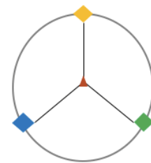
Figure 2: Quantitative Soil Pit Sampling Scheme
